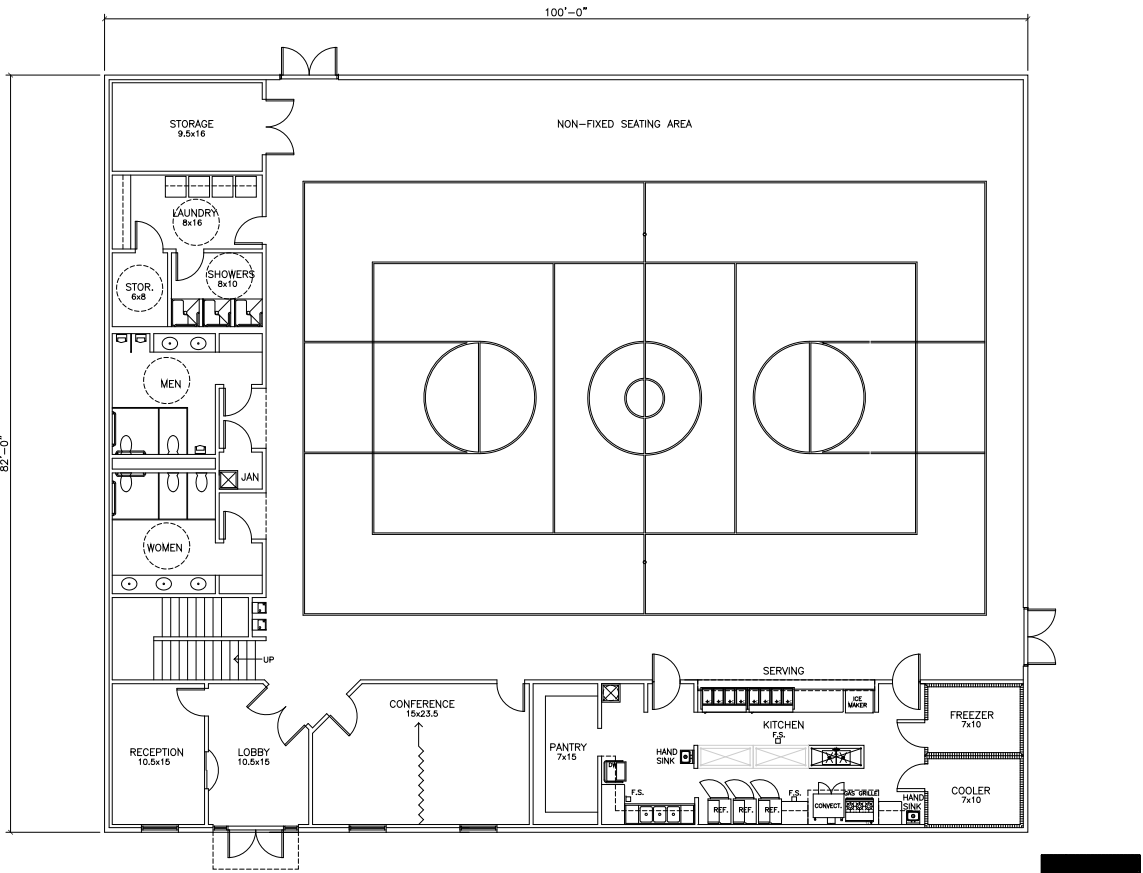
FIRST FLOOR PLAN BEAUTIFUL FEET MINISTRIES
