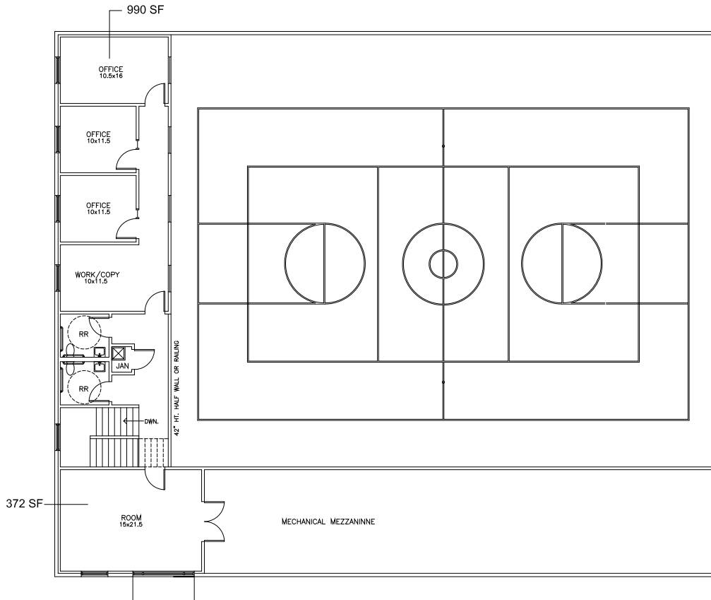
SECOND FLOOR PLAN BEAUTIFUL FEET MINISTRIES
